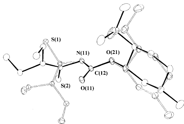
Fig. 3 Molecular structures of molecules 1 and 2 of N,N -diethyl- N' -(–)-(3 R )-menthylloxycarbonylthiourea superimposed. Molecule 2 is numbered with the first digit referring to the number of the molecule and the second to the number of the atom. Hydrogen atoms have been omitted for clarity.
