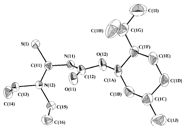
Fig. 2 Molecular structure showing the atom numbering scheme and displacement ellipsoids (30% probability) for molecule 1 of N,N -diethyl- N' -(−)-(3 R )-menthyloxy-carbonylthiourea 1 . Hydrogen atoms have been omitted for clarity.
